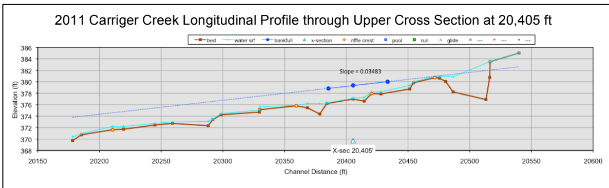
Figure 54. Estimated gradient is shown of the Carriger Creek streambed thalweg and bankfull flow at Cross Section 20,405 ft in the perennial reach downstream stream of the Grove Street box culvert.
