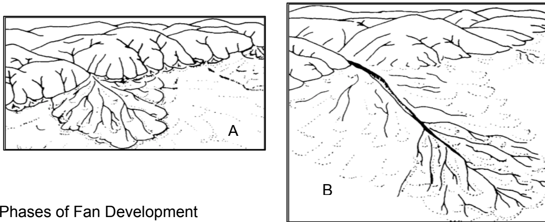
Figure 2. Two phases in the development of alluvial fans under the influence of tectonic uplift are shown. Figure A shows the area of deposition adjacent to the mountain front. Figure B shows the area of deposition shifted down fan due to stream channel entrenchment (from Leece (1990) with permission to reproduce from Bull. 196R).
