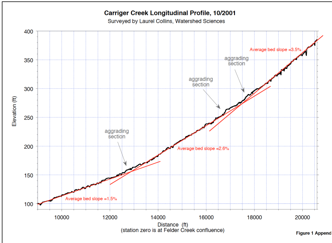
Figure 21. Red lines are shown to represent average gradient on this 2001 longitudinal profile. Collins et al (2002) suggested that long-term channel aggradation might occur at the locations where the red lines cross over each other. The crossover areas occur at major inflection points along the profile, Source: Collins et al 2002.
